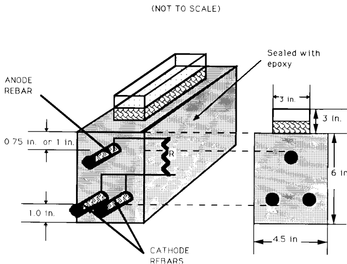
NOTE—All measurements in in. (25.4 mm = 1 in.). FIG. 1 Concrete Beam
