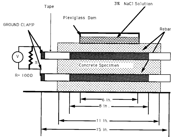
NOTE—All measurements in in. (not to scale) (25.4 mm = 1 in.). FIG. 2 Concrete Beam (Side View)
