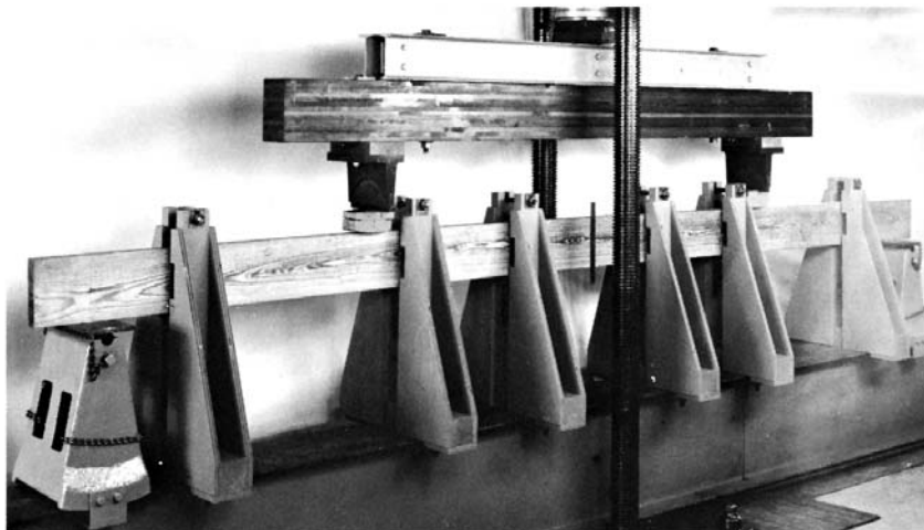
FIG. 2 Example of Lateral Support for Long, Deep Beams
