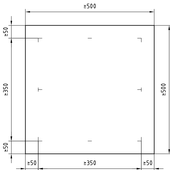
Figure 1 — Marking of fabric specimens (standards.iteh.ai)
