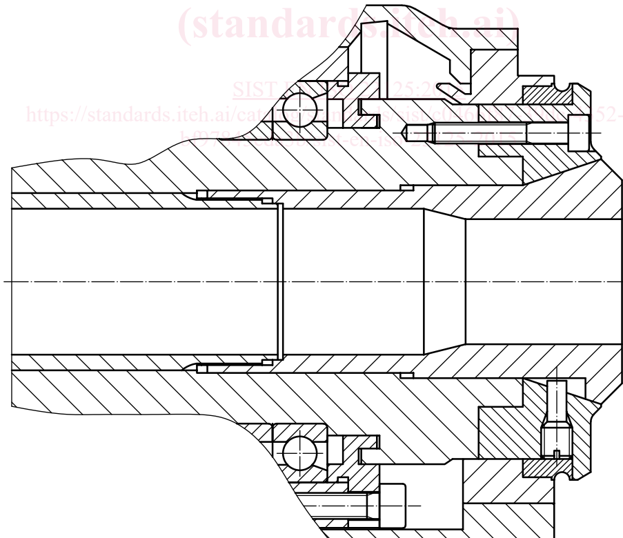
Figure 2 — Collet
