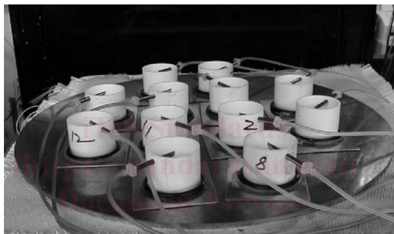
FIG. 3 Test Coupons on Hot Plate
