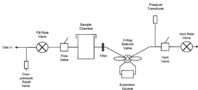
FIG. 1 Schematic Diagram of Gas Pycnometer
