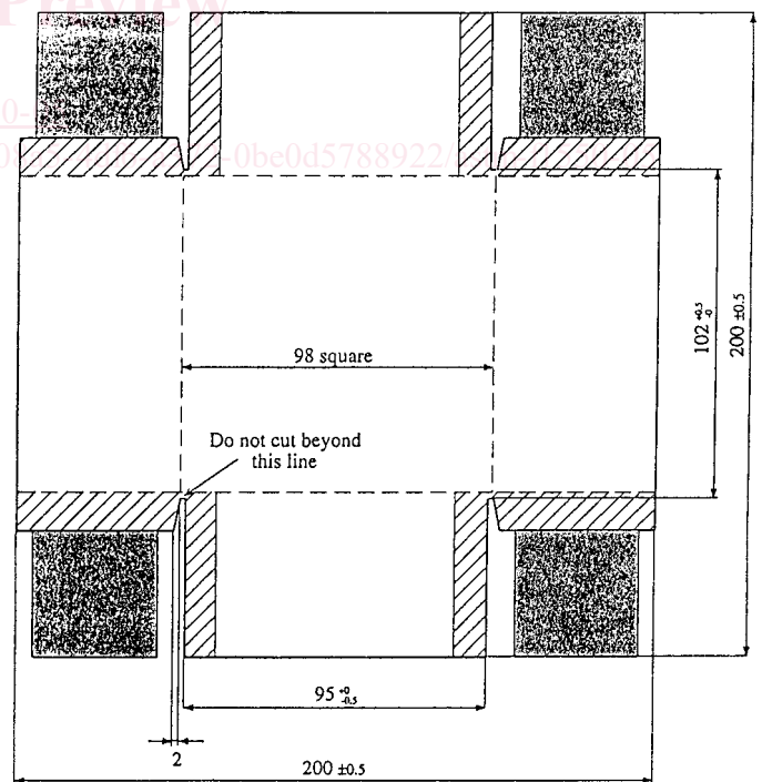
Gluing area To be cut off after gluing Dimensions in mm
