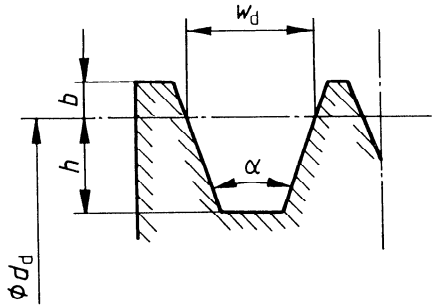
Figure 1 — Groove profile
