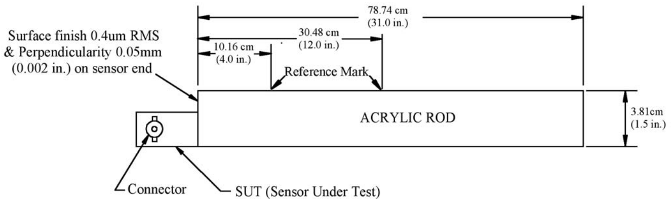
FIG. 1 Acrylic Rod Description
