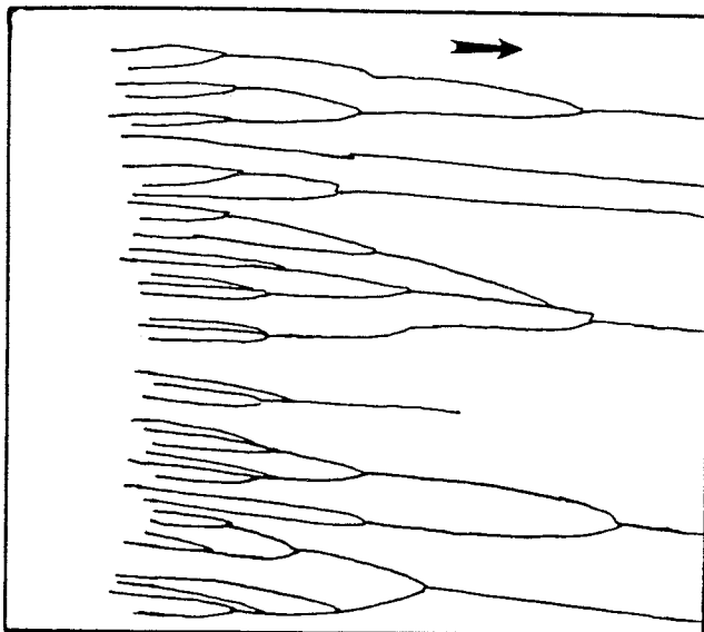
NOTE 1—The direction of crack propagation is shown by the arrow. FIG. 4 Schematic of Twist Hackle Lines That Form a “River Pattern”
