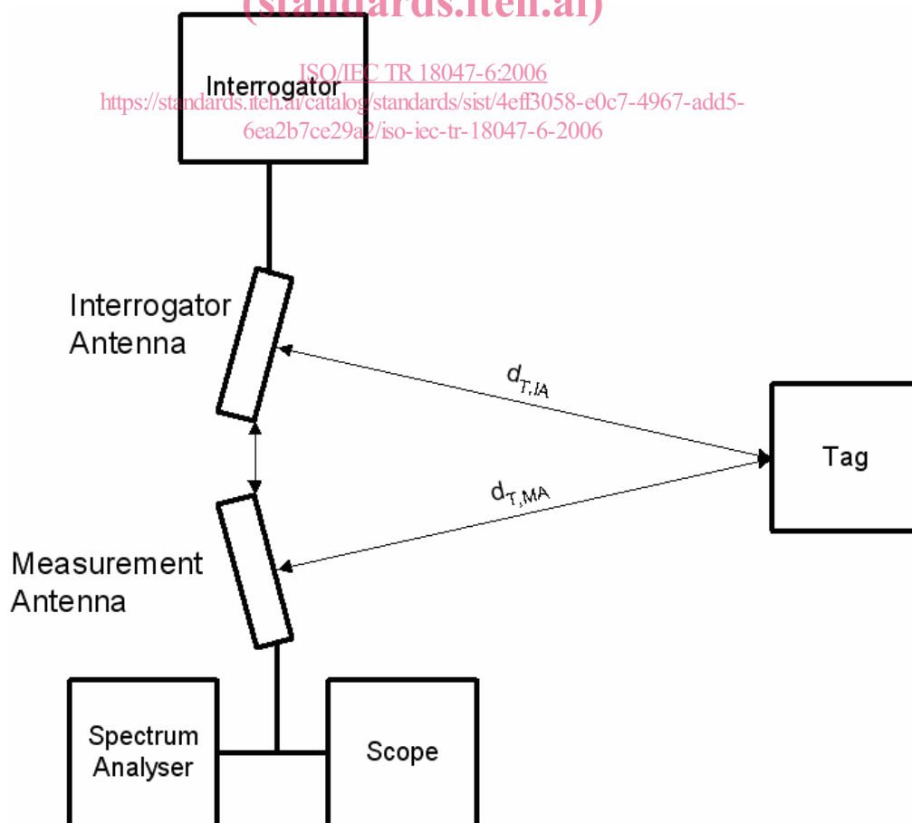
Figure 3 — Tag demodulation test setup
