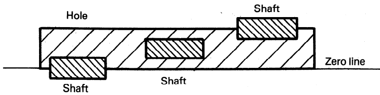
Figure 10 – Schematic representation of transition fits
