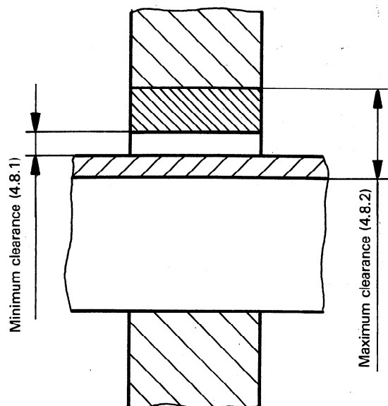
Figure 4 — Clearance fit
