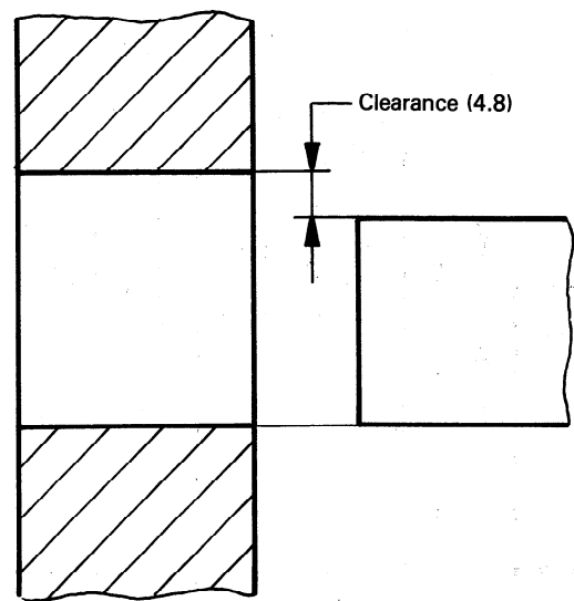
Figure 3 — Clearance
