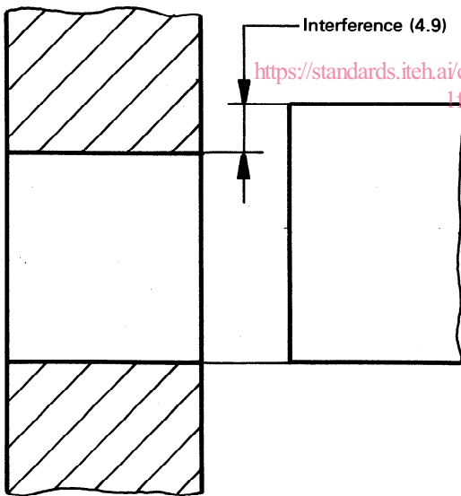
Figure 6 – Interference
