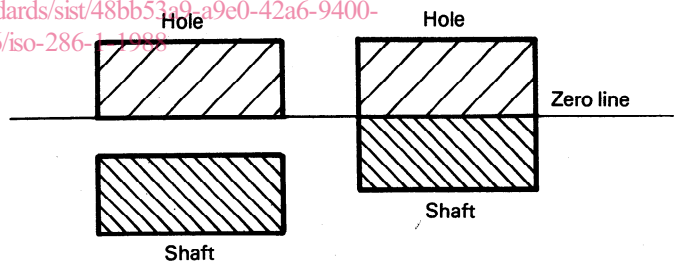
Figure 8 – Schematic representation of clearance fits
