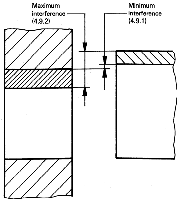
Figure 7 – Interference fit
