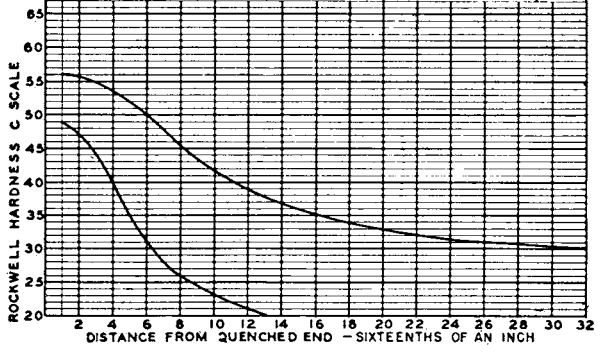
FIG. 2 Limits for Hardenability Band 1330 H
