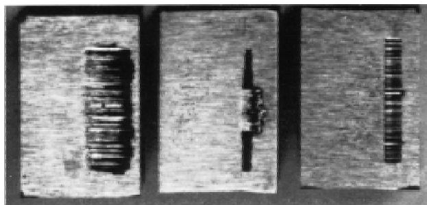
FIG. 1 Test Blocks Showing Various Types of Scar
