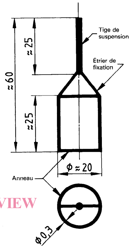
Figure 3 – Anneau [5.2 c)]
