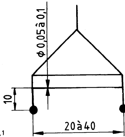
Figure 2 – Étrier [5.2 b)]
