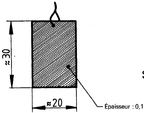
Figure 1 – Lame [5.2 a)]
