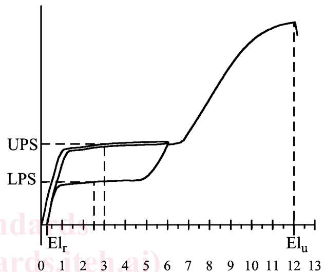
FIG. 1 Terms Illustrated on Typical Stress-Strain Diagram of Superelastic Nitinol
