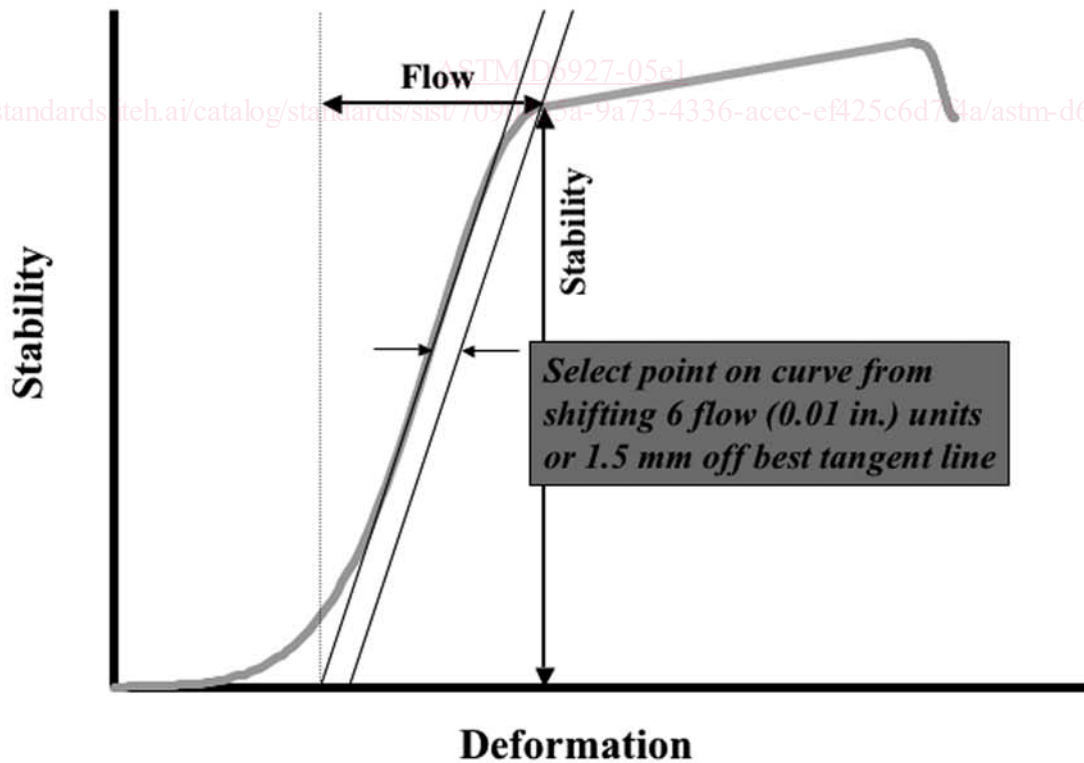
FIG. 1 Flow Determination for Two Types of Specimen Failure
