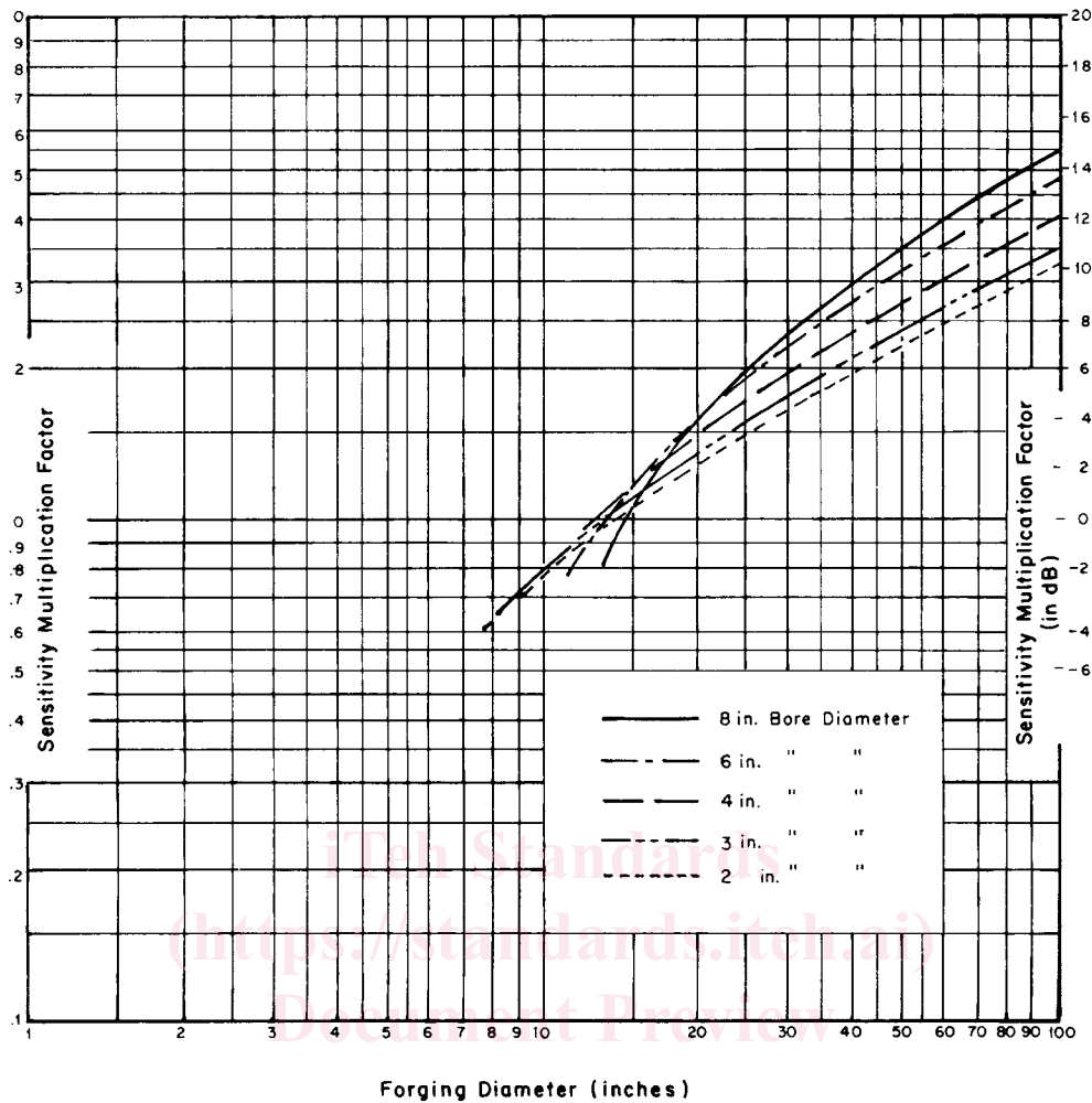
ASTM A418/A418M-05 SENSITIVITY MULTIPLICATION FACTORS FOR BORED FORGINGS
