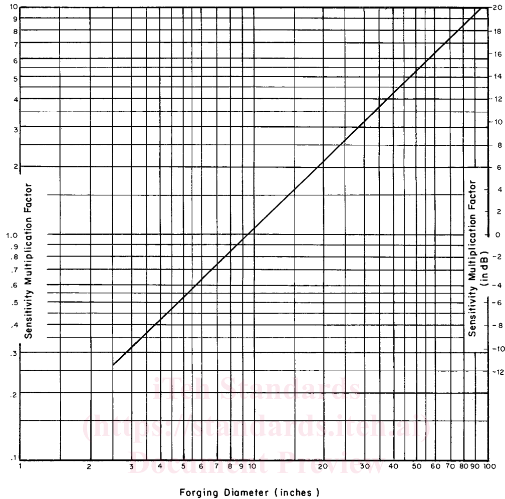
ASTM A418/A418M-05 SENSITIVITY MULTIPLICATION FACTORS FOR SOLID FORGINGS
