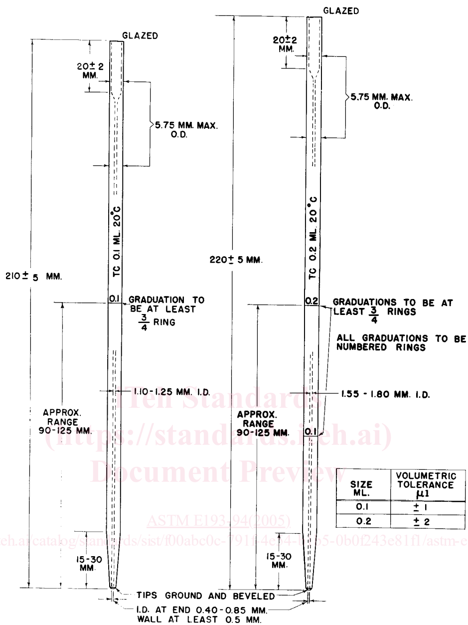
FIG. 2 Micropipets, Folin-Type
