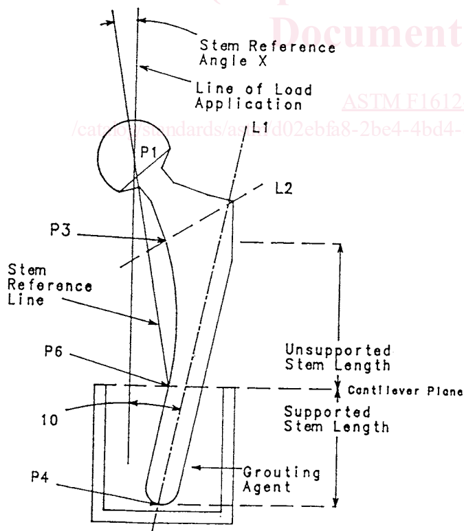
FIG. 2 1(b) Collarless Device, M-L Projection
