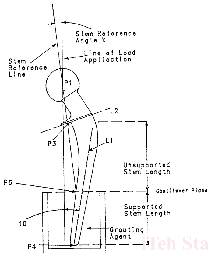
FIG. 1 1(a) Collared Device, M-L Projection
