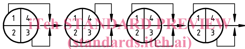
Figure 1 — Sampling procedure for granulated scrap and turnings
