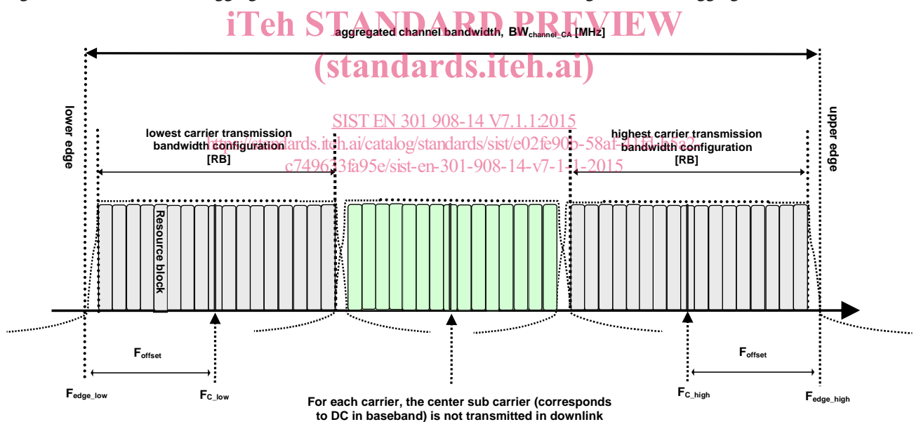
Figure 3.1-2: Aggregated channel bandwidth for intra-band carrier aggregation
