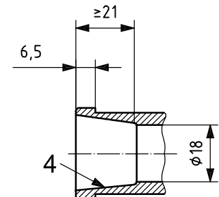
c) Female component — Taper and socket (only essential dimensions shown) a
