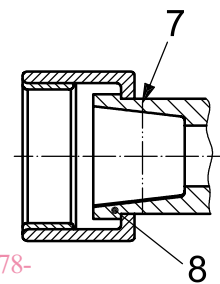
c) Female component — Taper and socket (only essential dimensions shown) a
