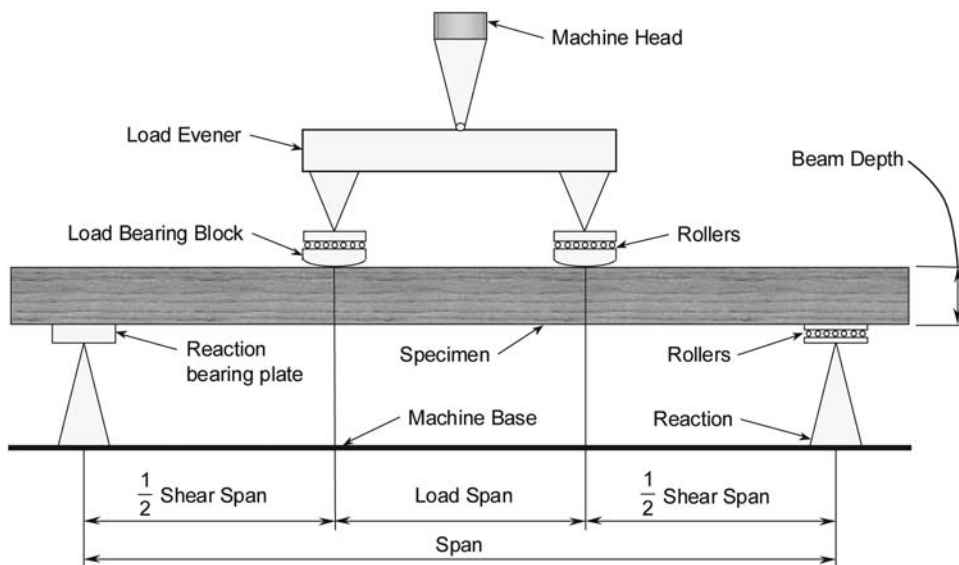
FIG. 1 Flexure Method. Example of Two-Point Loading
