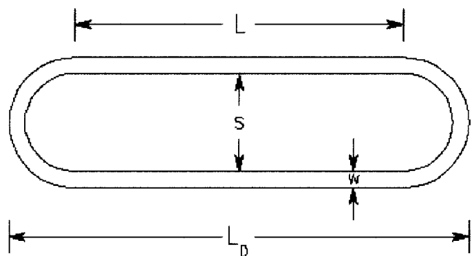
FIG. 2 Schematic of Link-Type Lamination
