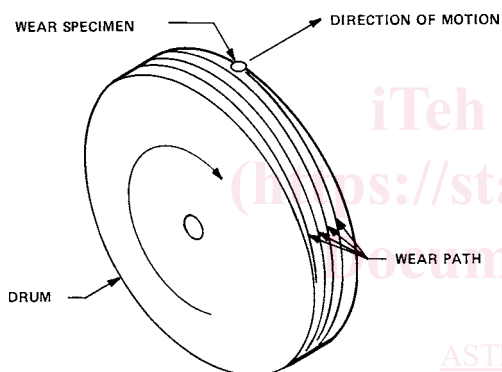
FIG. 2 Test Motion
