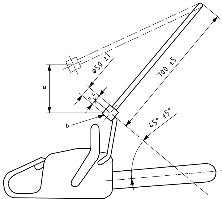
Figure 1 — Impact direction and pendulum (standards.iteh.ai)
