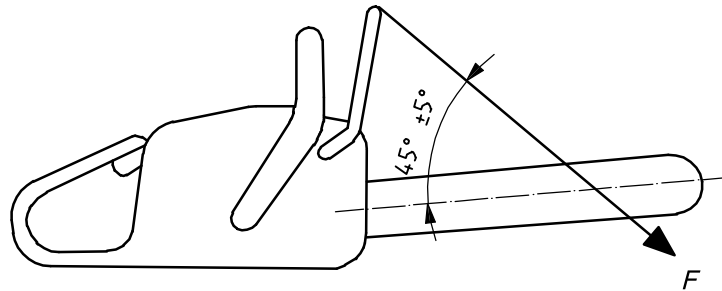
Figure 2 — Measuring direction for release force, F
