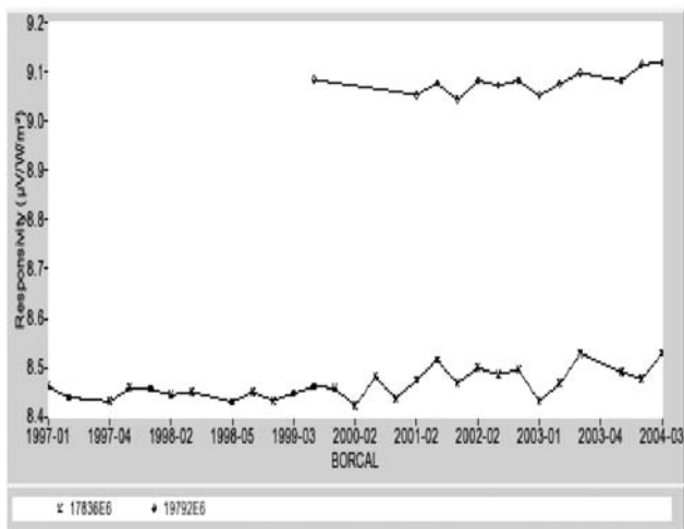
NOTE—Each graph shows repeated calibration results for two pyrheliometers.
