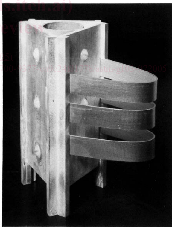
U bend specimens (Practice G39) stressed in an anodized aluminum fixture (right photo) are placed in a pyrex battery jar (left photo), which is placed over a magnetic stirrer. The 6 % salt solution is heated to boiling by means of two quartz immersion heaters. A powerstat controls the heat output of the quartz heaters. A cold water circulating aluminum condenser tube is placed just below the aluminum cover to prevent evaporation losses. Stressed specimens are placed in the jar after the solution comes to a boil. Specimens are examined in place for visual evidence of cracking.
