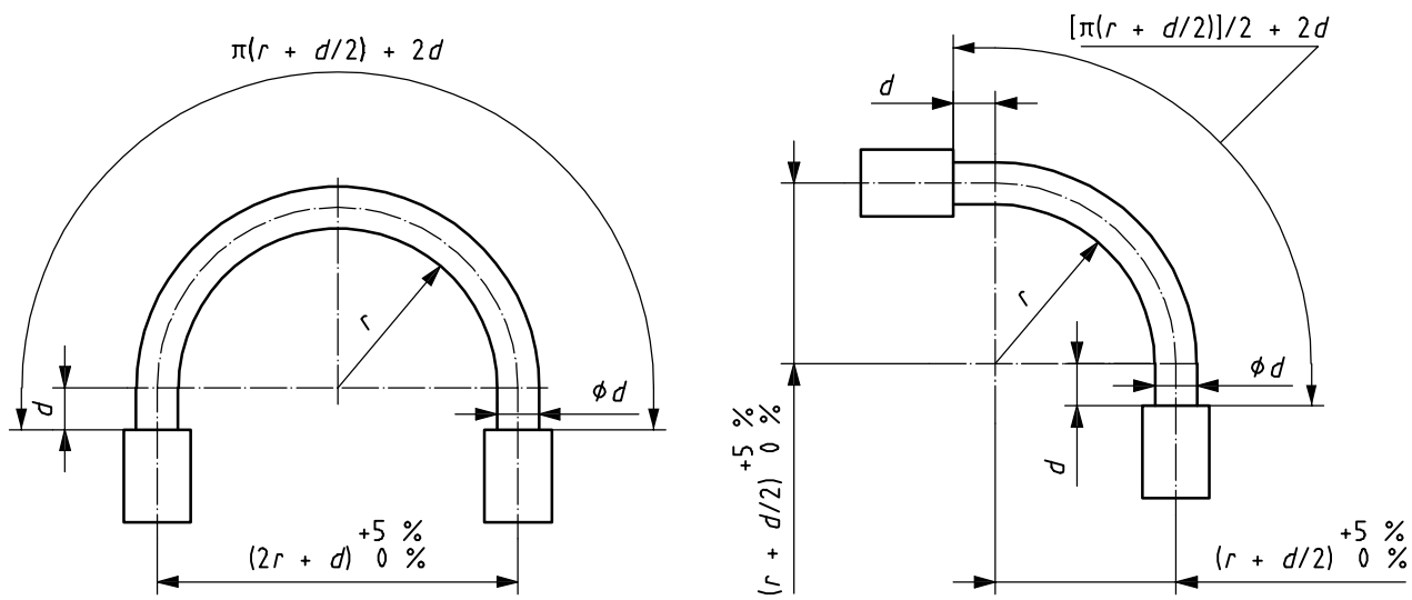
a) Hose sizes up to and including 22 mm nominal inside diameter
