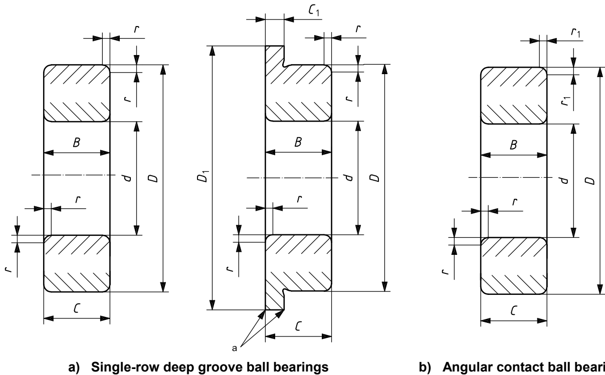
iTeh STANDARD PREVIEW (standards.iteh.ai) Figure 1 — Instrument precision bearing
