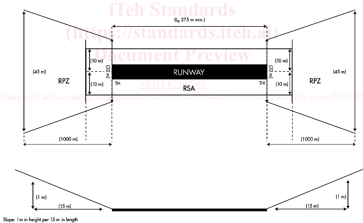
FIG. 1 Runway Length—Threshold
