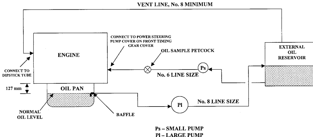
FIG. A1.1 Auxiliary Oil System
