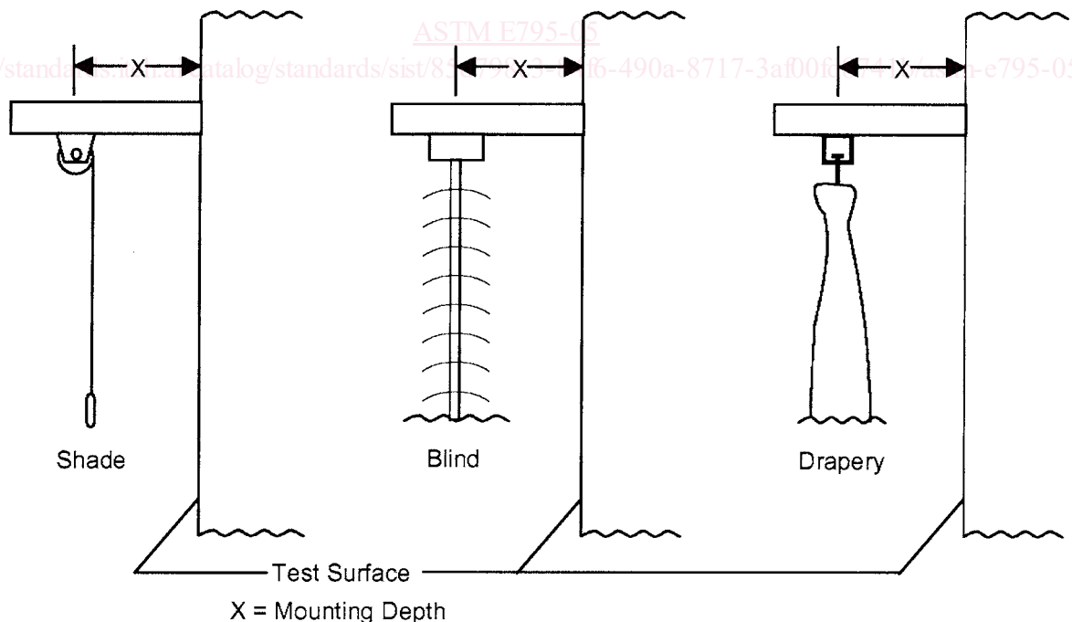
FIG. 8 Type G Mounting
