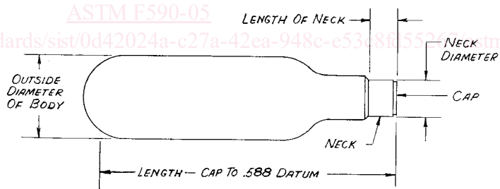
CO 2 (CARBON DIOXIDE) CYLINDER
