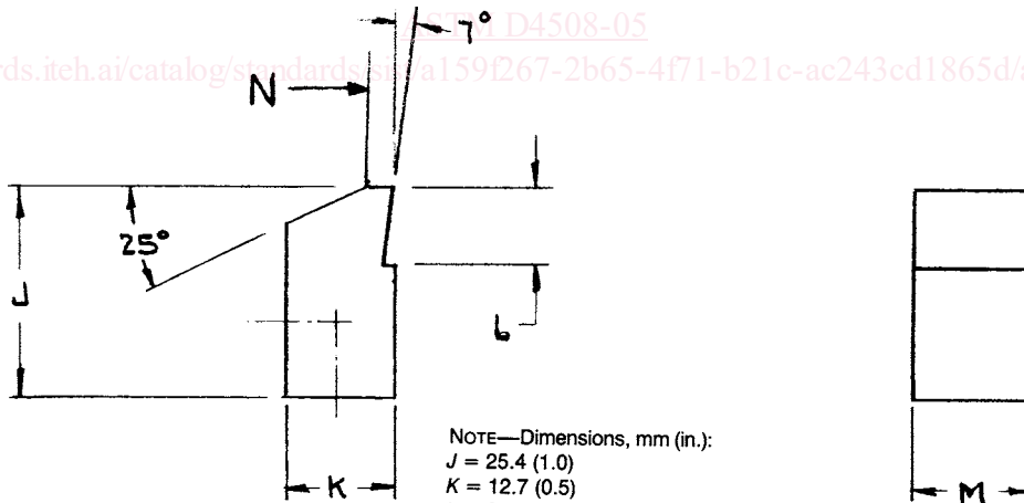
FIG. 1 Specimen Holder
