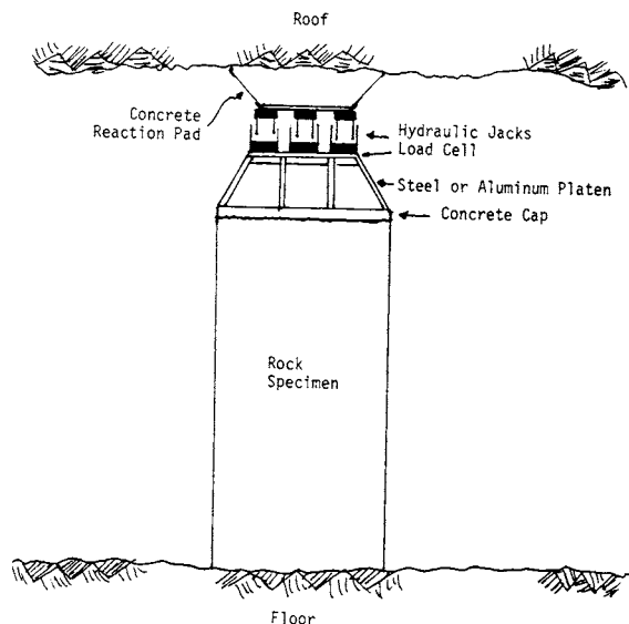
FIG. 2 Test Arrangement
