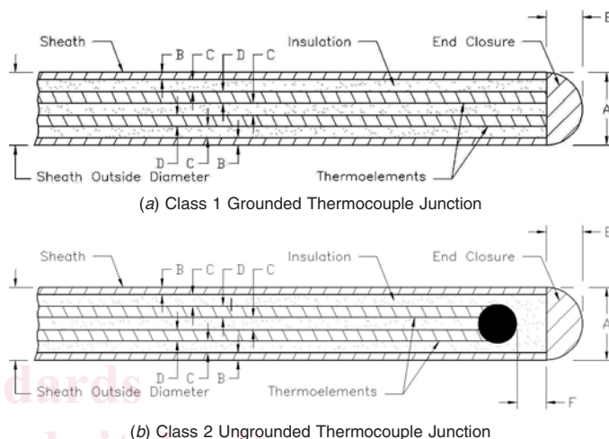
FIG. 3 Sheathed Thermocouple Assembly
