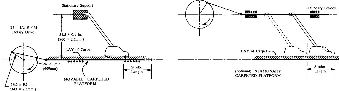
FIG. 1 Test Fixture
