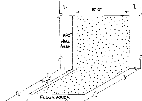
FIG. 2 Concrete Wall and Floor Test Area
