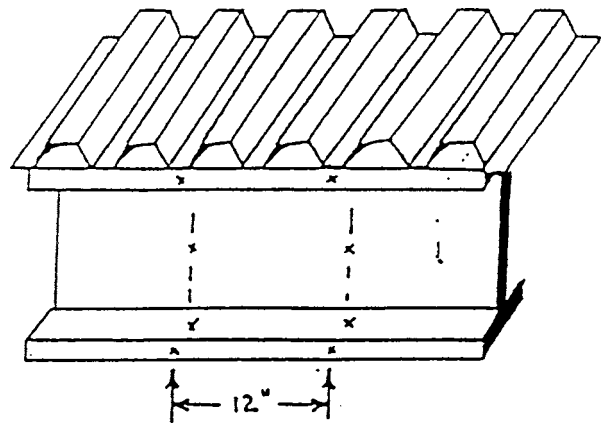
NOTE—Take nine measurements at each end of 12 in. length. FIG. 3 Beam
