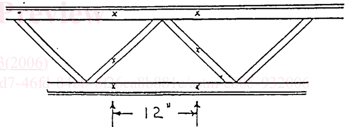
NOTE—Take 7 measurements at each end of 12 in. length. FIG. 5 Joist
