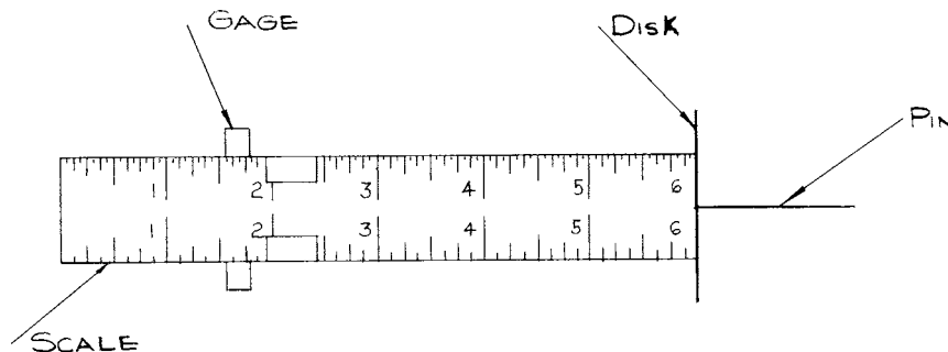
FIG. 1 Thickness Gage
