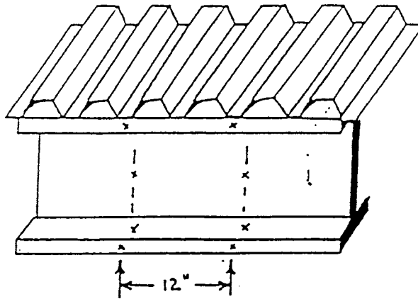
FIG. 3 Beam
