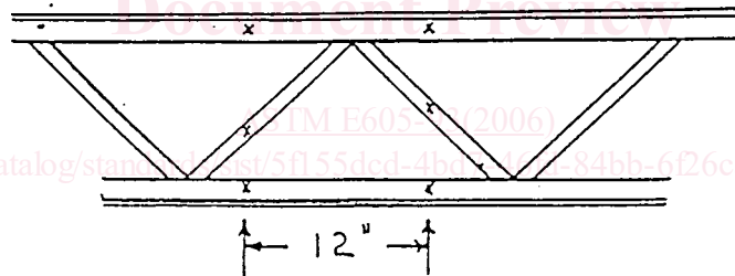
FIG. 5 Joist
