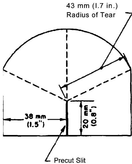
FIG. 1 Die or Template for Constant-Radius Test Specimen
