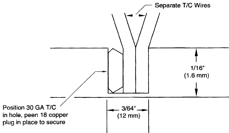
FIG. 6 Thermocouple Wire Installation
