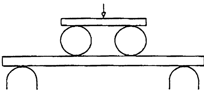
FIG. 1 Four Point Loading and Support Noses at Maximum Radius
