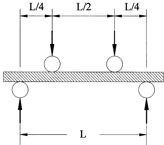
FIG. 2 Four-Point-¼ Point Flexural Test Fixture Configuration
