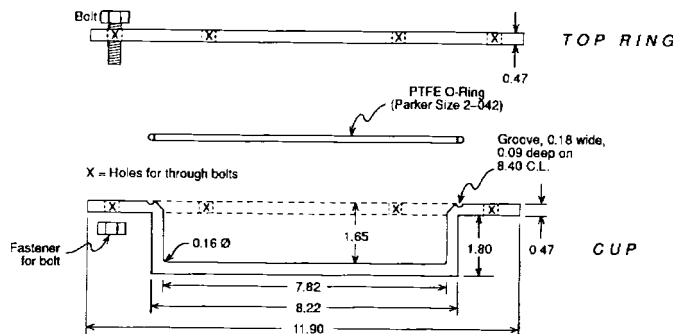
FIG. 1 ASTM Permeation Cup
