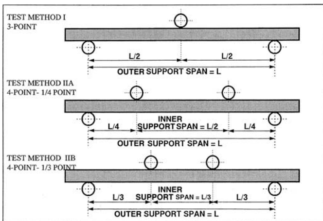
FIG. 1 Flexural Test Geometries
