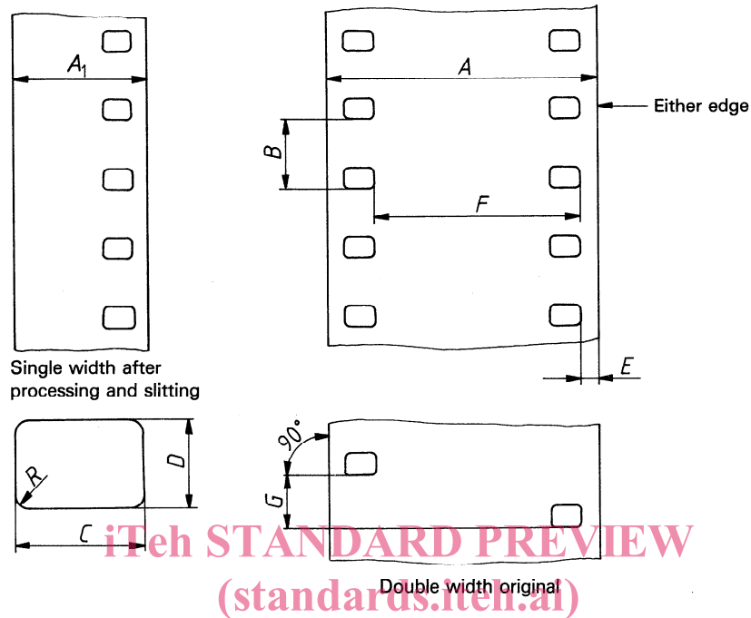
ISO 486:1988 https://standards.iteh.ai/catalog/standards/sist/cbb16485-0373-4679-8c9e-017a09969ccc/iso-486-1988 Figure — 16 mm film perforated 8 mm Type R
