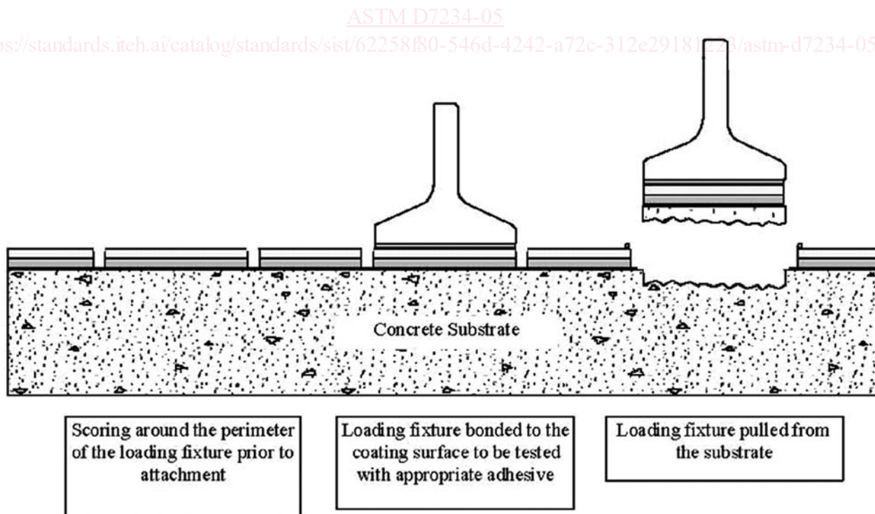
FIG. 1 Scoring Around the Loading Fixture Prior to Attachment of the Fixture (Round Loading Fixtures)
